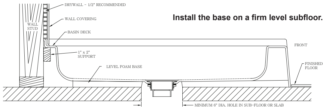
FIGURE 1 TYPICAL CROSS SECTION VIEW
