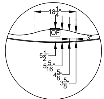
Faucet Deck Flat Dimensions
