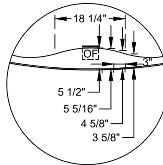
Faucet Deck Flat Dimensions
