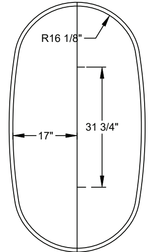
Drop In Hole Size
