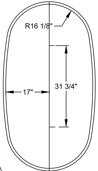
Drop In Hole Size
