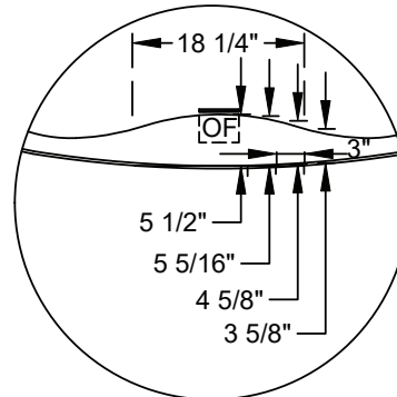
Faucet Deck Flat Dimensions
