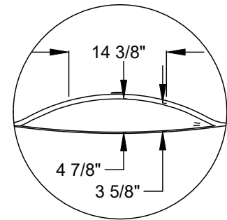
Faucet Deck Flat Dimensions
