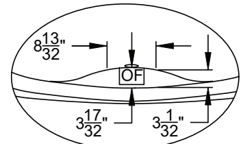
Faucet Deck Flat Dimensions
