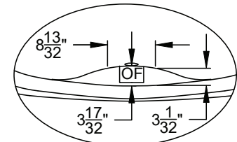
Faucetry Deck Flat Dimensions
