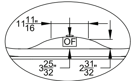
Faucetry Deck Flat Dimensions
