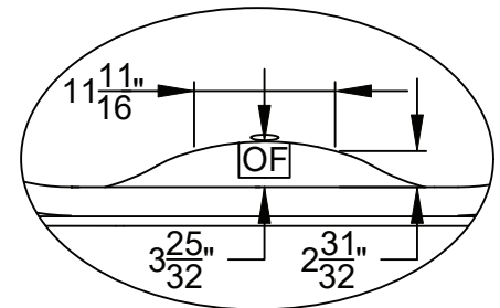
Faucet Deck Flat Dimensions
