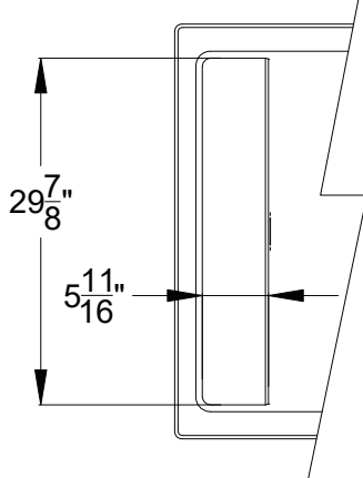
Faucetry Deck Flat Dimensions
