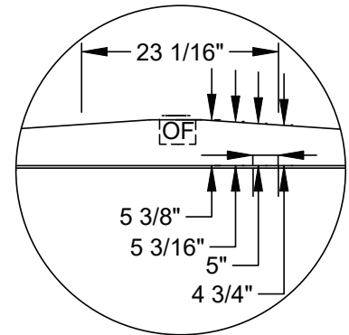
Faucet Deck Flat Dimensions
